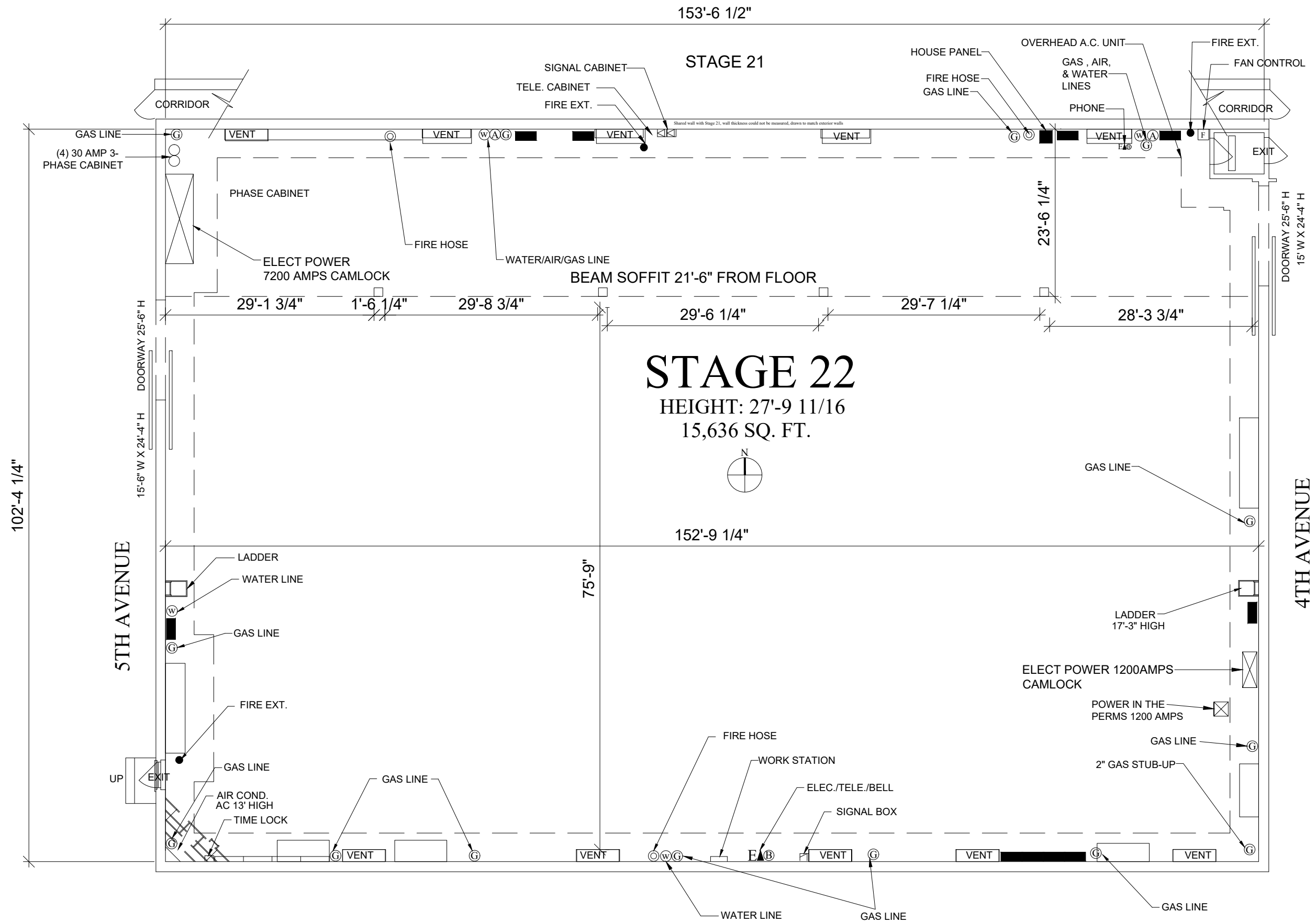
STAGE AREA DIAGRAM
